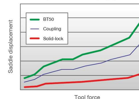
Comparison of tool clamping system
